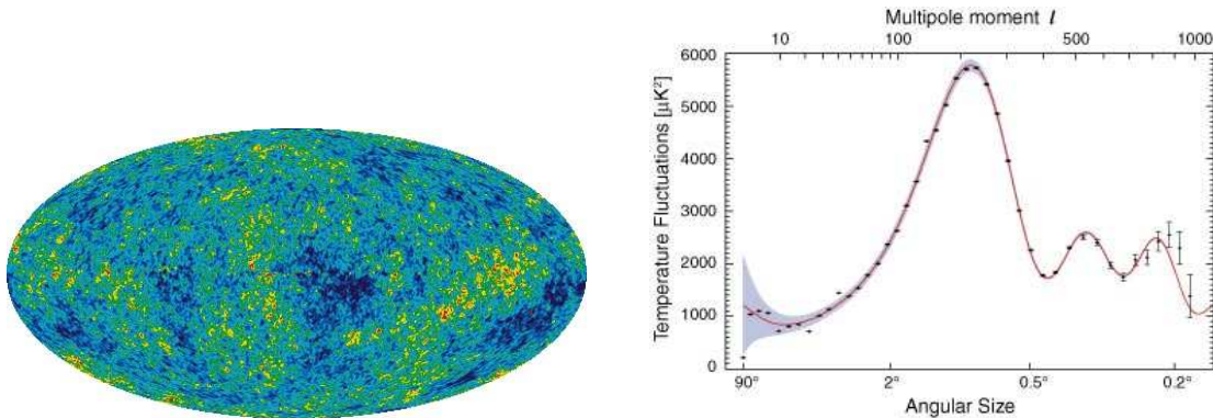
Figure 6: WMAP data.
