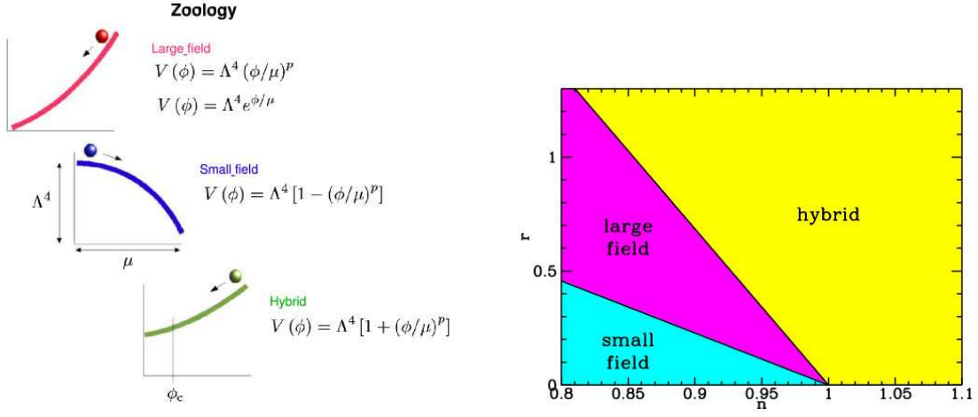
Figure 7: Inflationary models.
